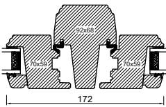
MULLION
