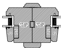
VERTICAL COUPLING
