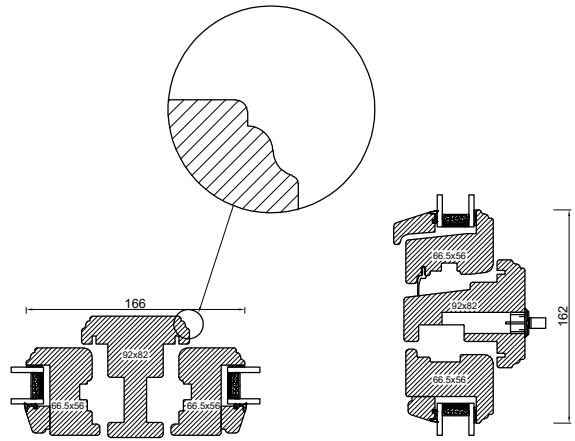
MULLION
