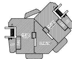
BAY COUPLING
