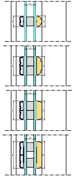
Glazing Bars L-L & M-M
